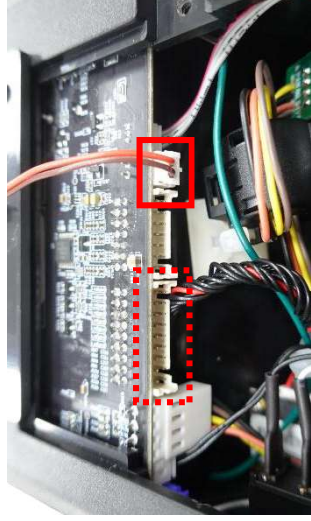
RTC connector (dotted line: Wireless connector position)
